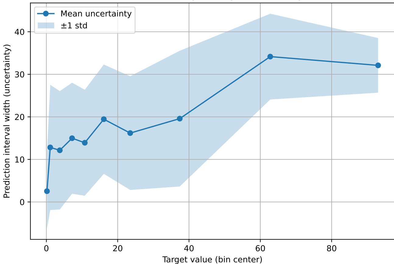
P2P: Uncertainty vs Target Value Range
